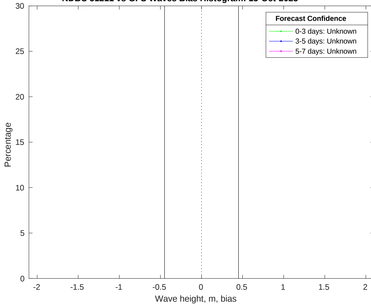
NDBC 51211 vs GFS Waves Bias Histogram: 15-Oct-2025
