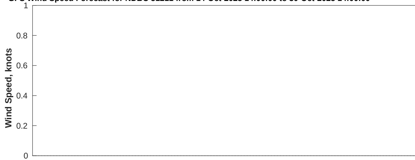
GFS Wind Speed Forecast for NDBC 51211 from 14-Oct-2025 14:00:00 to 30-Oct-2025 14:00:00
