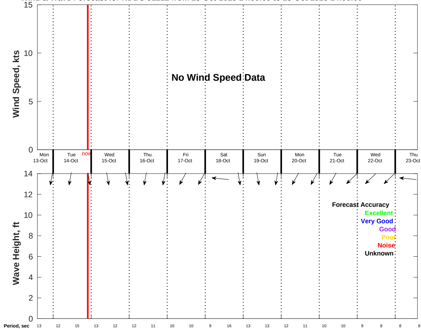
Wind & Wave Forecast for NDBC 51211 from 13-Oct-2025 14:00:00 to 23-Oct-2025 14:00:00
