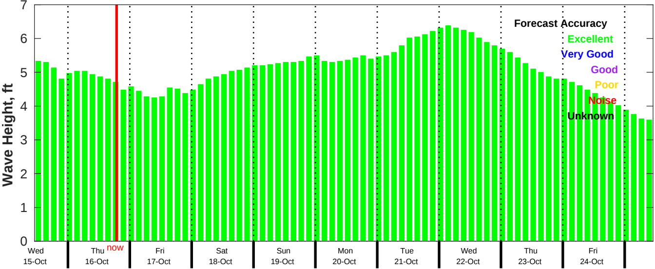
CMEMS Wave Forecast for NDBC 52211 from 14-Oct-2025 11:00:00 to 24-Oct-2025 11:00:00
