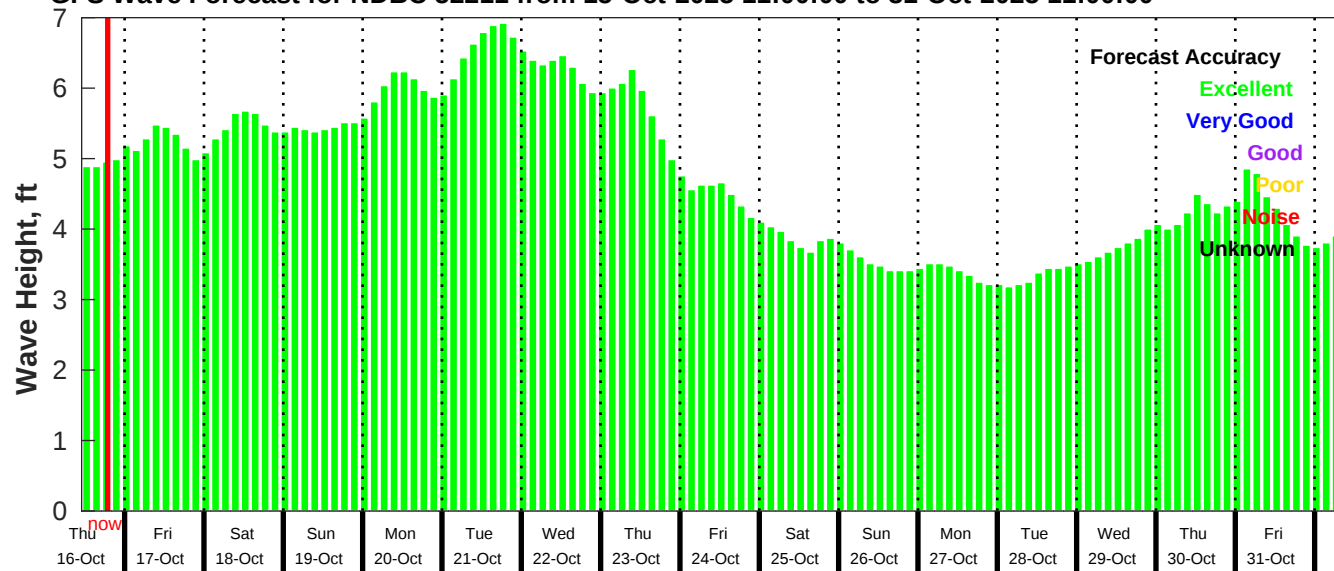
GFS Wave Forecast for NDBC 52211 from 15-Oct-2025 11:00:00 to 31-Oct-2025 11:00:00
