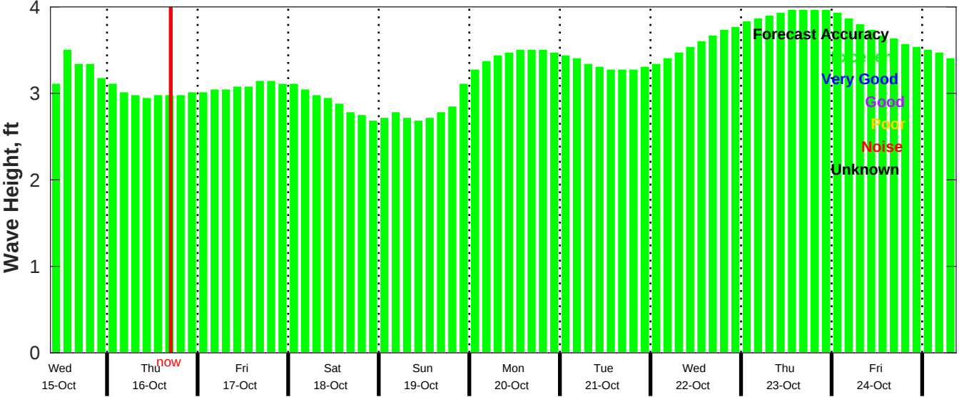
CMEMS Wave Forecast for NDBC 52212 from 14-Oct-2025 09:00:00 to 24-Oct-2025 09:00:00
