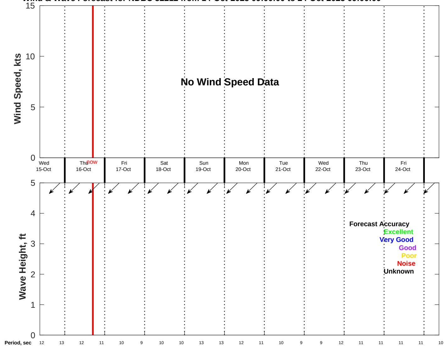
Wind & Wave Forecast for NDBC 52212 from 14-Oct-2025 09:00:00 to 24-Oct-2025 09:00:00
