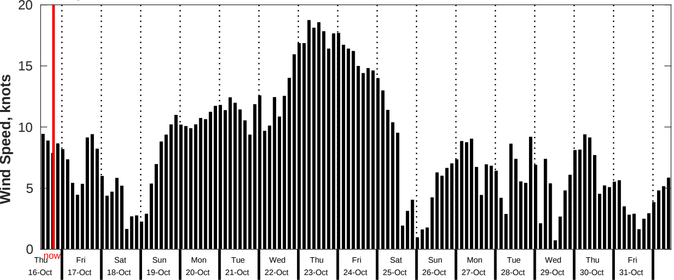
GFS Wind Speed Forecast for NDBC 52213 from 15-Oct-2025 11:00:00 to 31-Oct-2025 11:00:00
