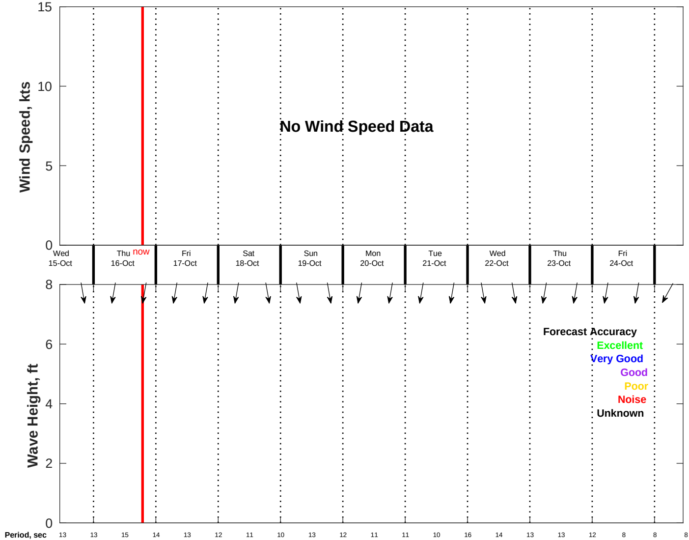
Wind & Wave Forecast for NDBC 52213 from 14-Oct-2025 11:00:00 to 24-Oct-2025 11:00:00
