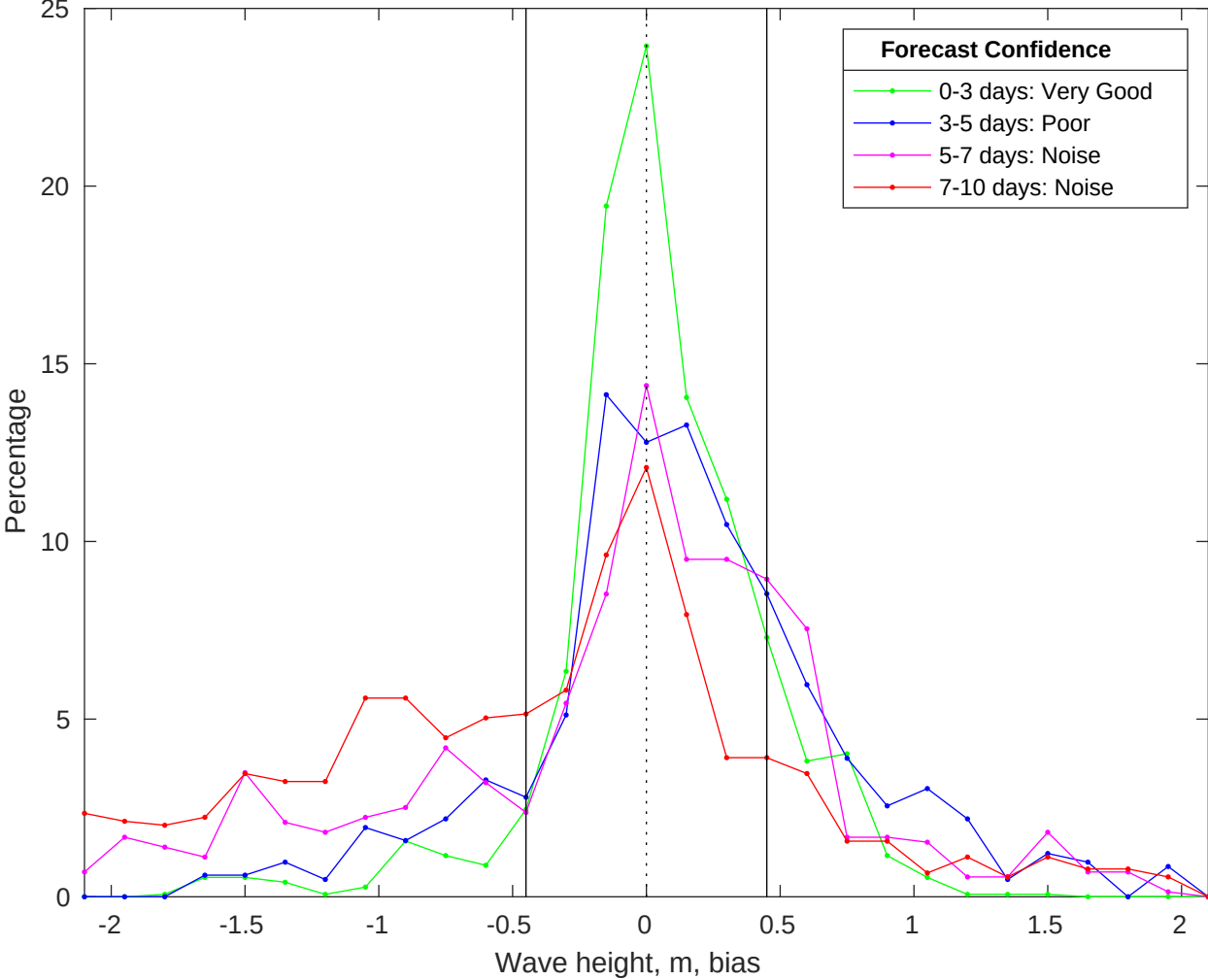
NDBC 41004 vs CMEMS Waves Bias Histogram: 16-Oct-2025
