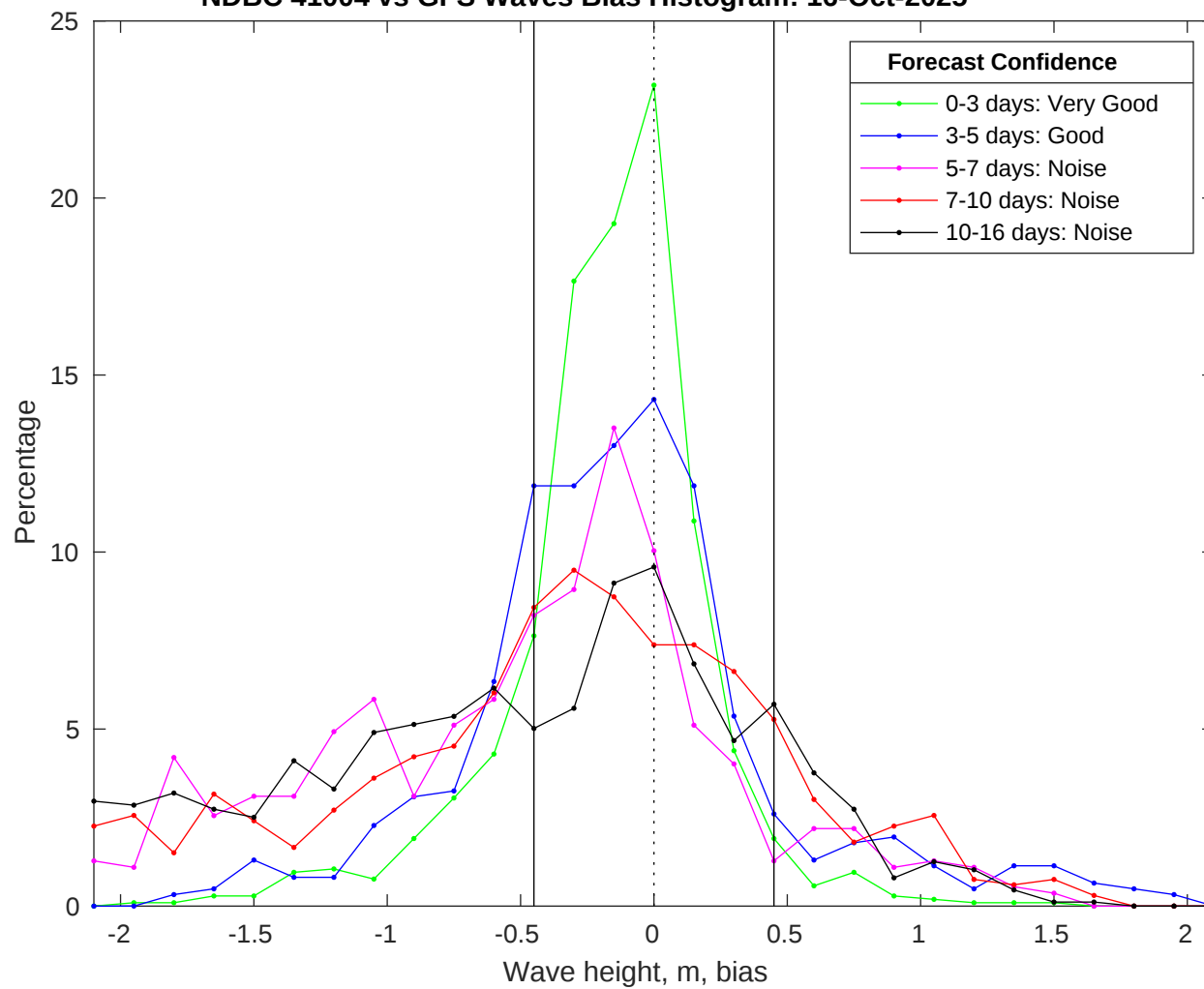
NDBC 41004 vs GFS Waves Bias Histogram: 16-Oct-2025
