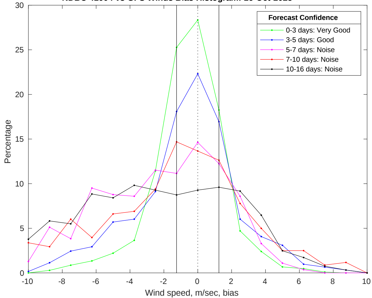
NDBC 41004 vs GFS Winds Bias Histogram: 16-Oct-2025
