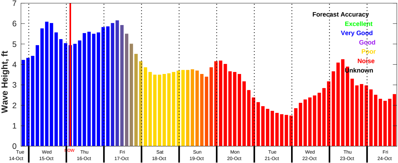
CMEMS Wave Forecast for NDBC 41004 from 14-Oct-2025 19:00:00 to 24-Oct-2025 19:00:00
