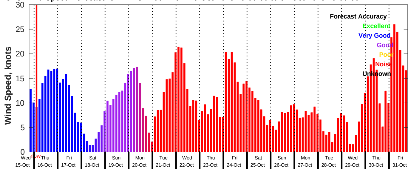
GFS Wind Speed Forecast for NDBC 41004 from 15-Oct-2025 19:00:00 to 31-Oct-2025 19:00:00
