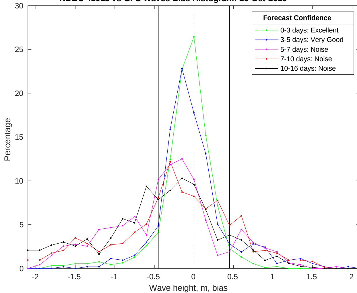
NDBC 41013 vs GFS Waves Bias Histogram: 16-Oct-2025
