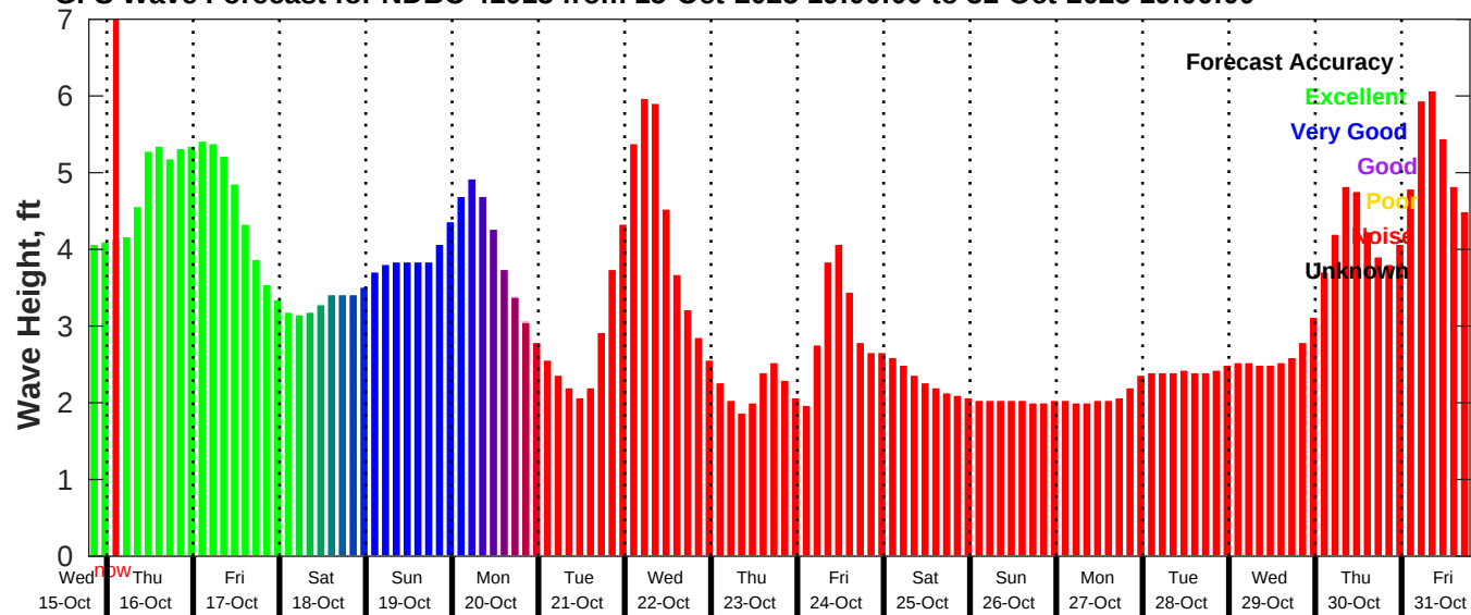
GFS Wave Forecast for NDBC 41013 from 15-Oct-2025 19:00:00 to 31-Oct-2025 19:00:00
