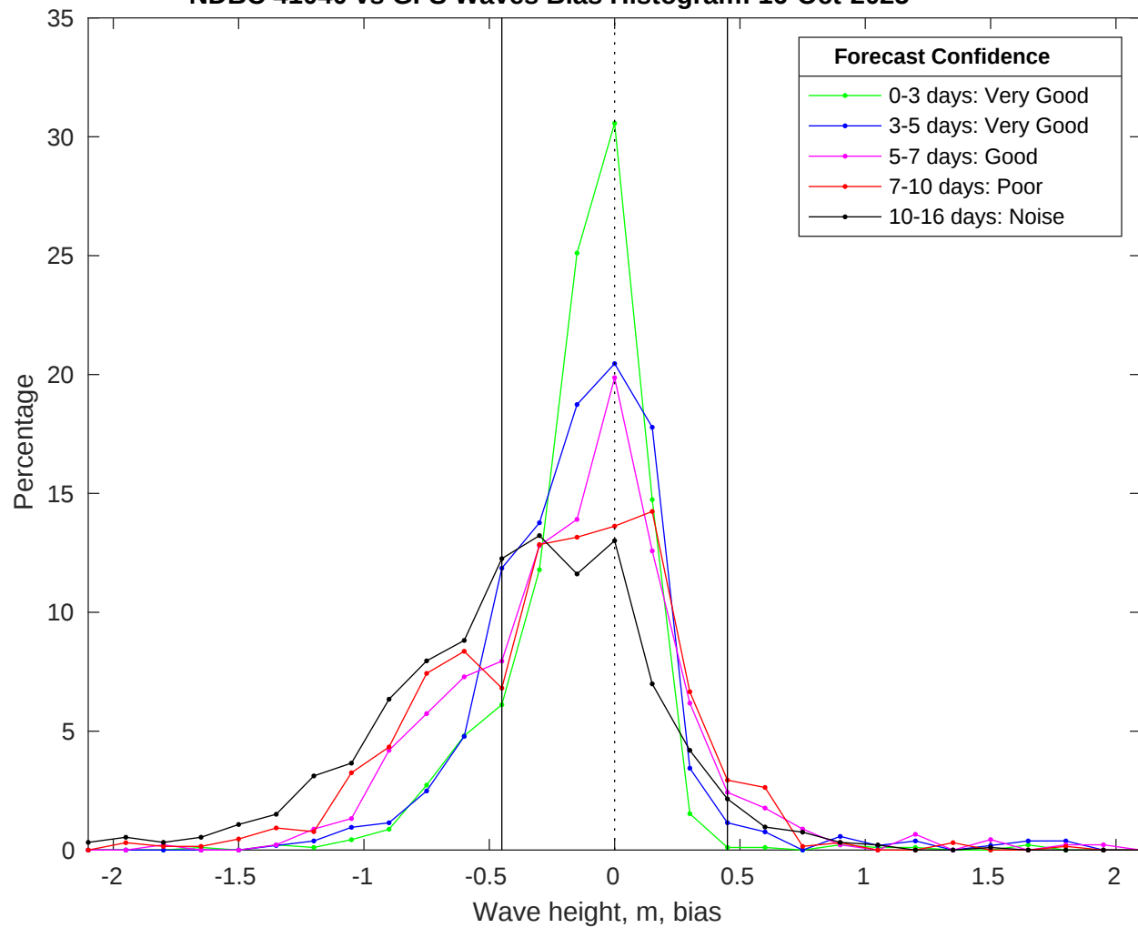
NDBC 41040 vs GFS Waves Bias Histogram: 16-Oct-2025
