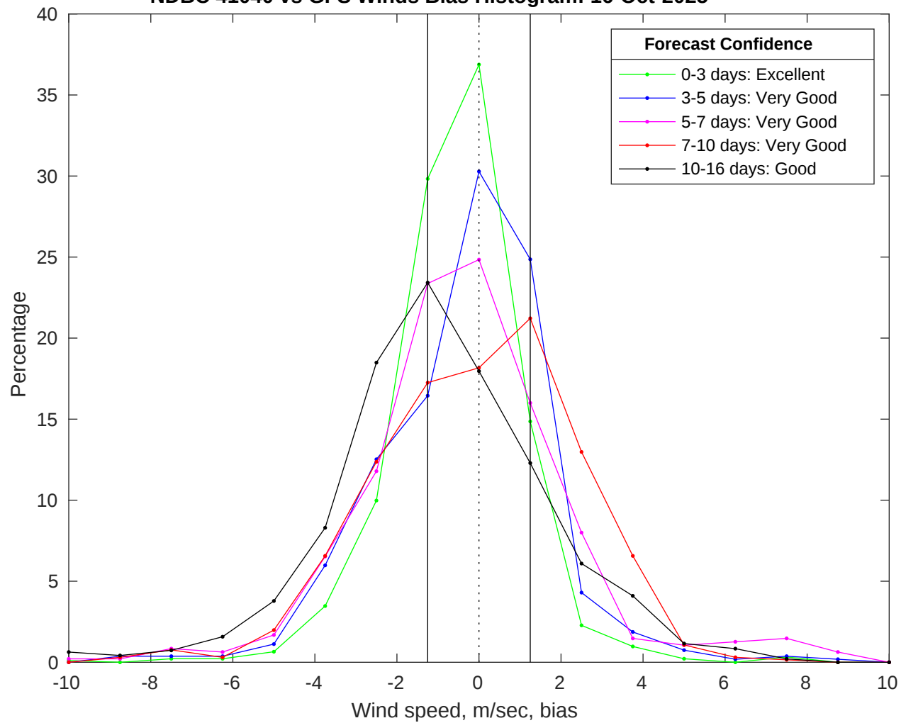
NDBC 41040 vs GFS Winds Bias Histogram: 16-Oct-2025
