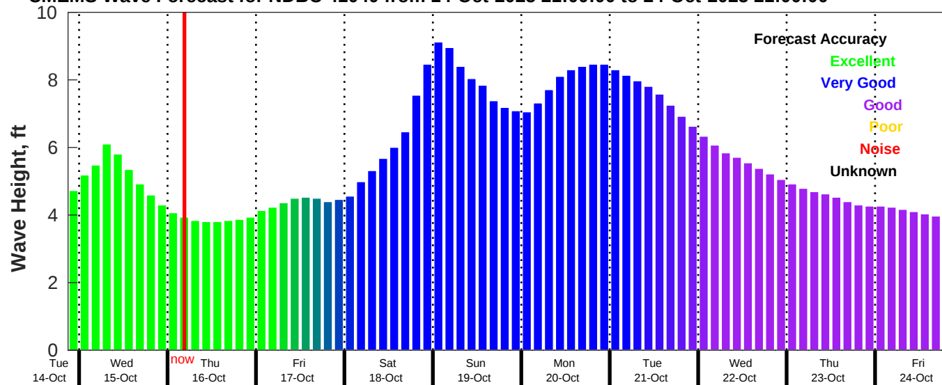
CMEMS Wave Forecast for NDBC 41040 from 14-Oct-2025 21:00:00 to 24-Oct-2025 21:00:00
