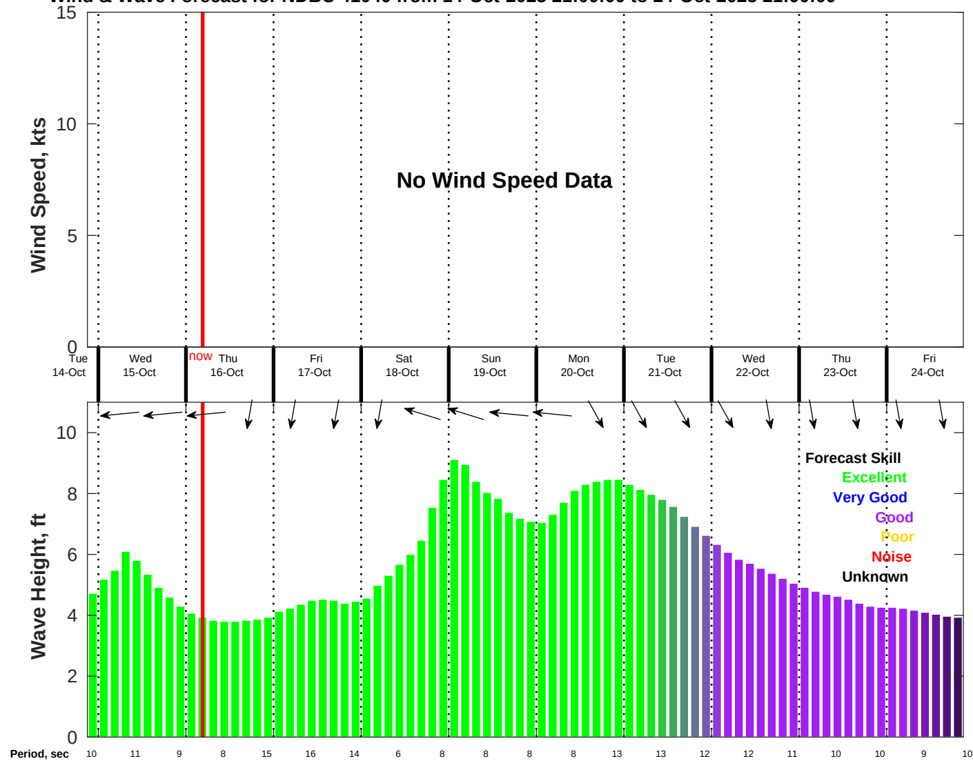
Wind & Wave Forecast for NDBC 41040 from 14-Oct-2025 21:00:00 to 24-Oct-2025 21:00:00
