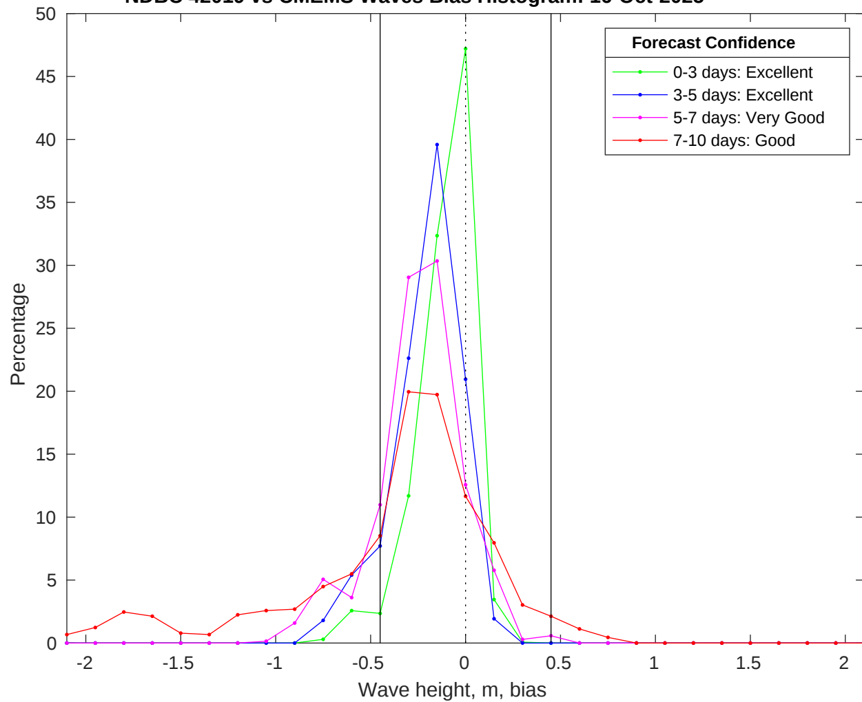
NDBC 42019 vs CMEMS Waves Bias Histogram: 16-Oct-2025
