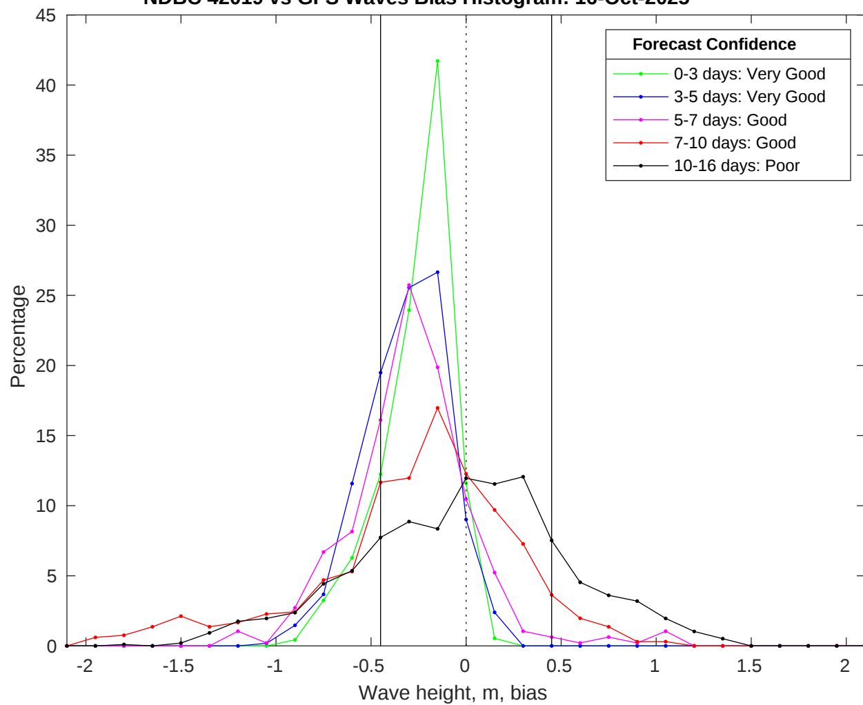
NDBC 42019 vs GFS Waves Bias Histogram: 16-Oct-2025
