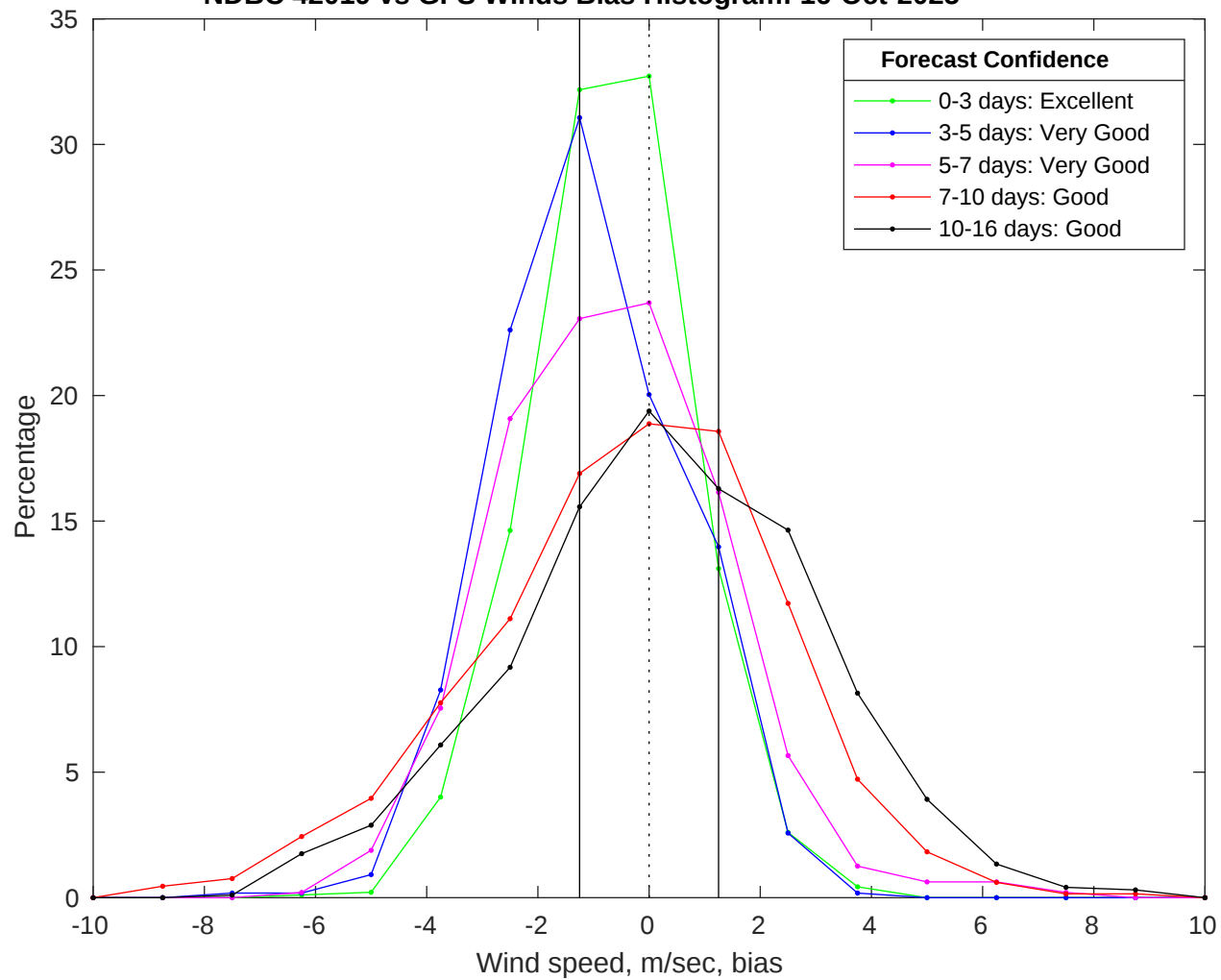
NDBC 42019 vs GFS Winds Bias Histogram: 16-Oct-2025
