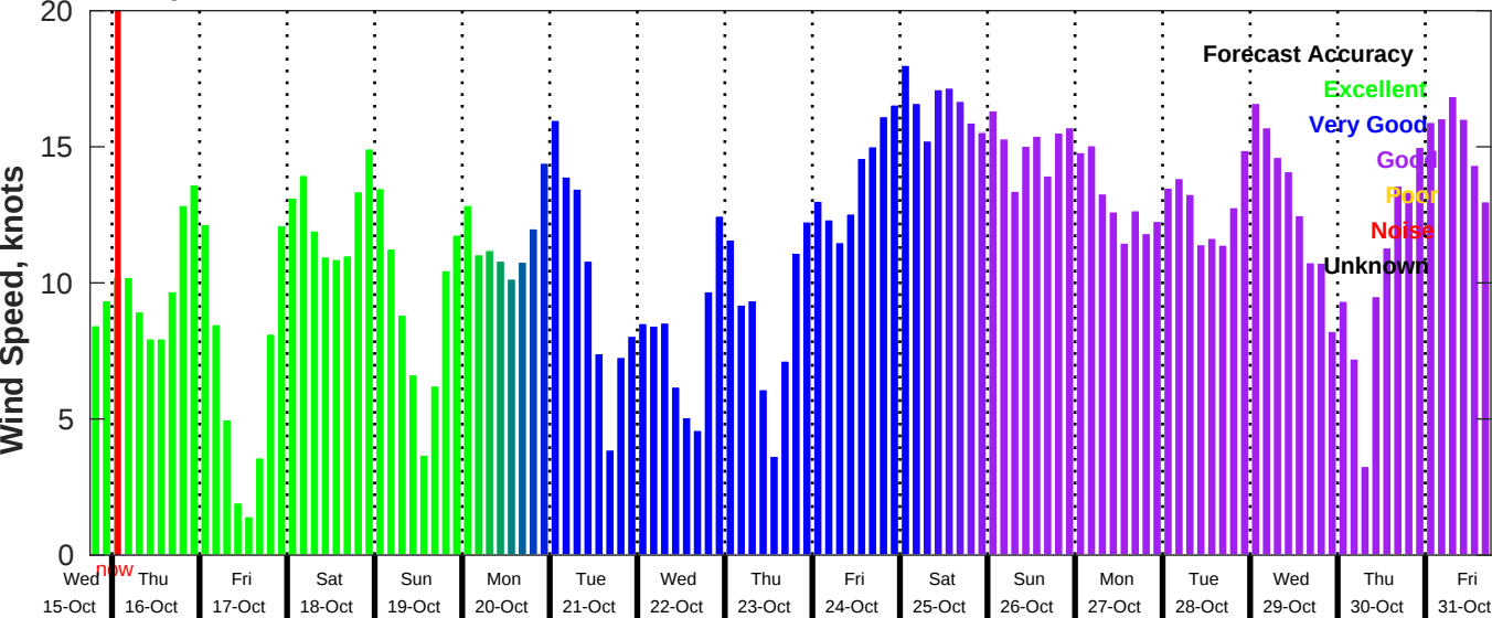
GFS Wind Speed Forecast for NDBC 42020 from 15-Oct-2025 18:00:00 to 31-Oct-2025 18:00:00
