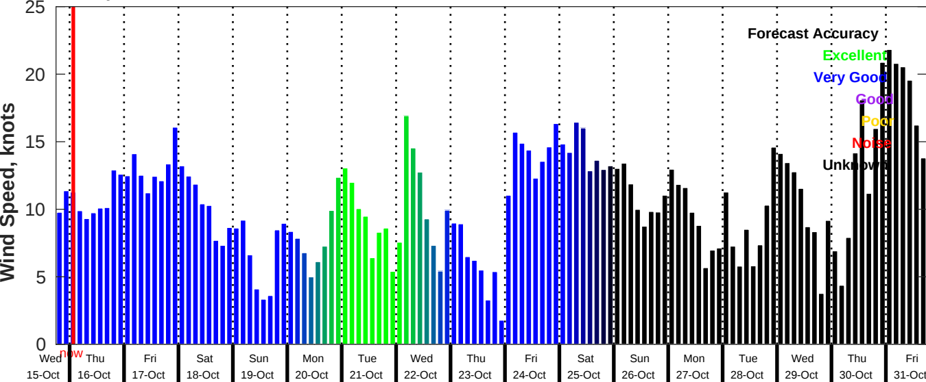
GFS Wind Speed Forecast for NDBC 42035 from 15-Oct-2025 18:00:00 to 31-Oct-2025 18:00:00
