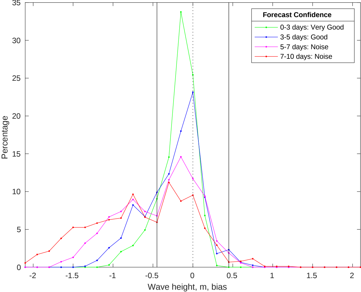
NDBC 42036 vs CMEMS Waves Bias Histogram: 16-Oct-2025
