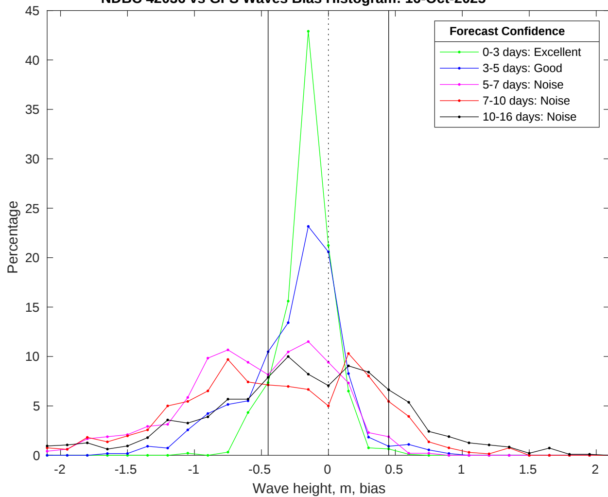
NDBC 42036 vs GFS Waves Bias Histogram: 16-Oct-2025
