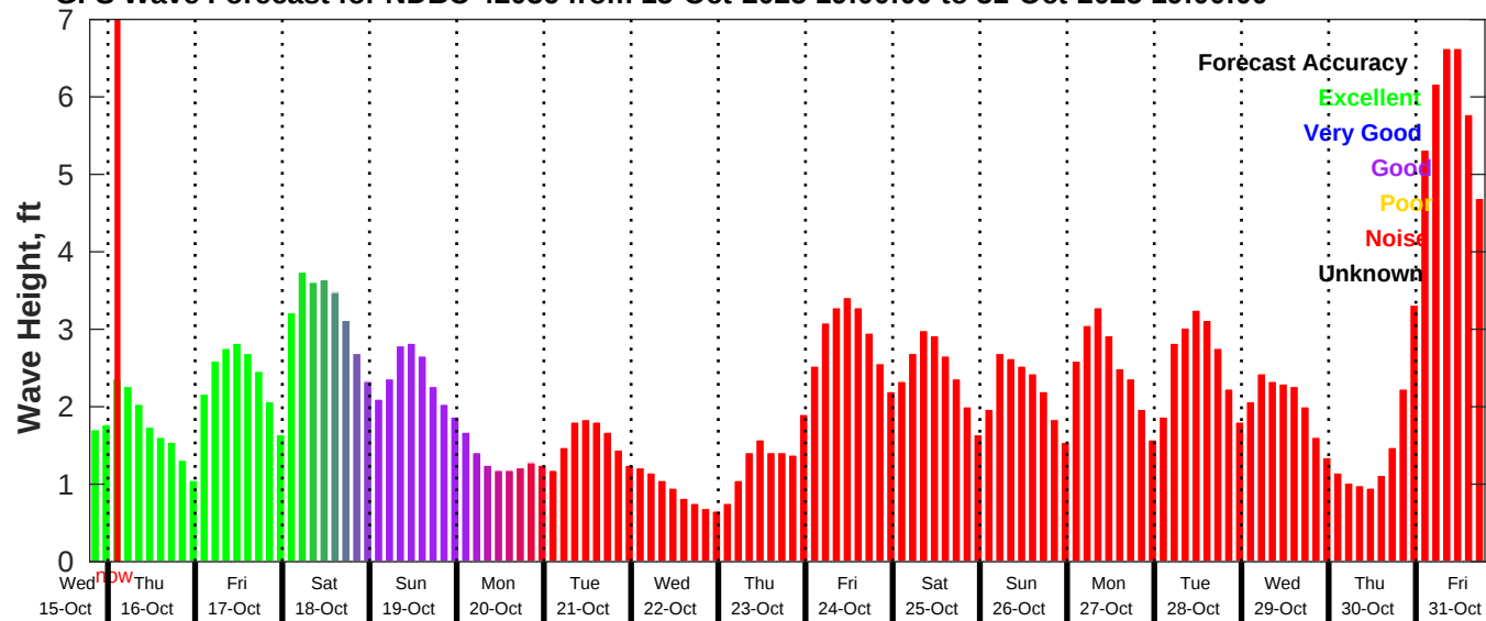
GFS Wave Forecast for NDBC 42036 from 15-Oct-2025 19:00:00 to 31-Oct-2025 19:00:00
