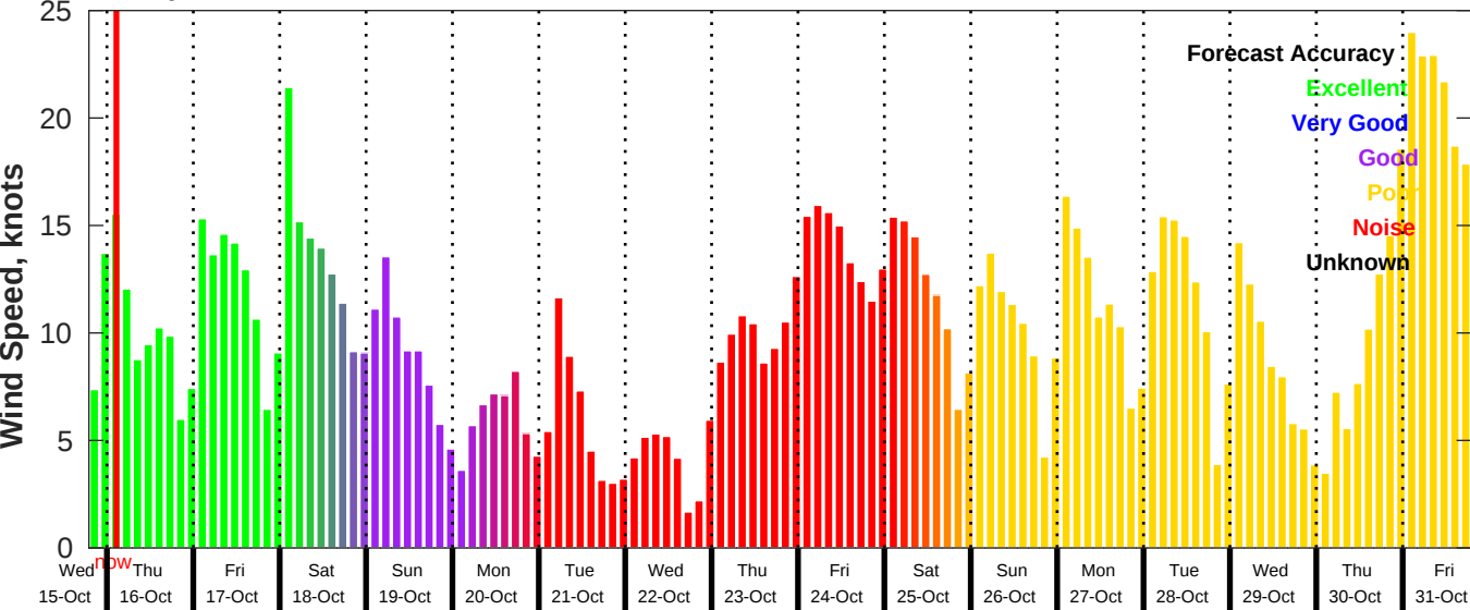
GFS Wind Speed Forecast for NDBC 42036 from 15-Oct-2025 19:00:00 to 31-Oct-2025 19:00:00
