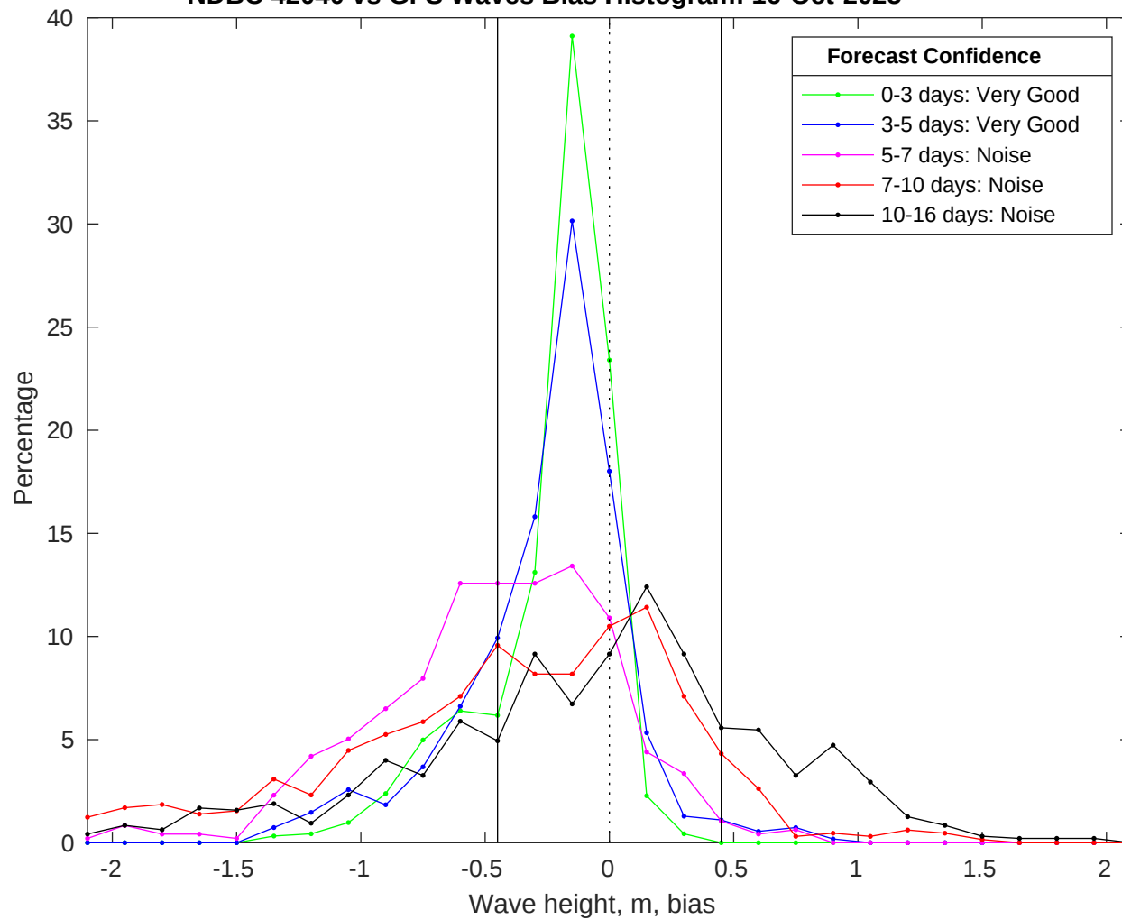
NDBC 42040 vs GFS Waves Bias Histogram: 16-Oct-2025
