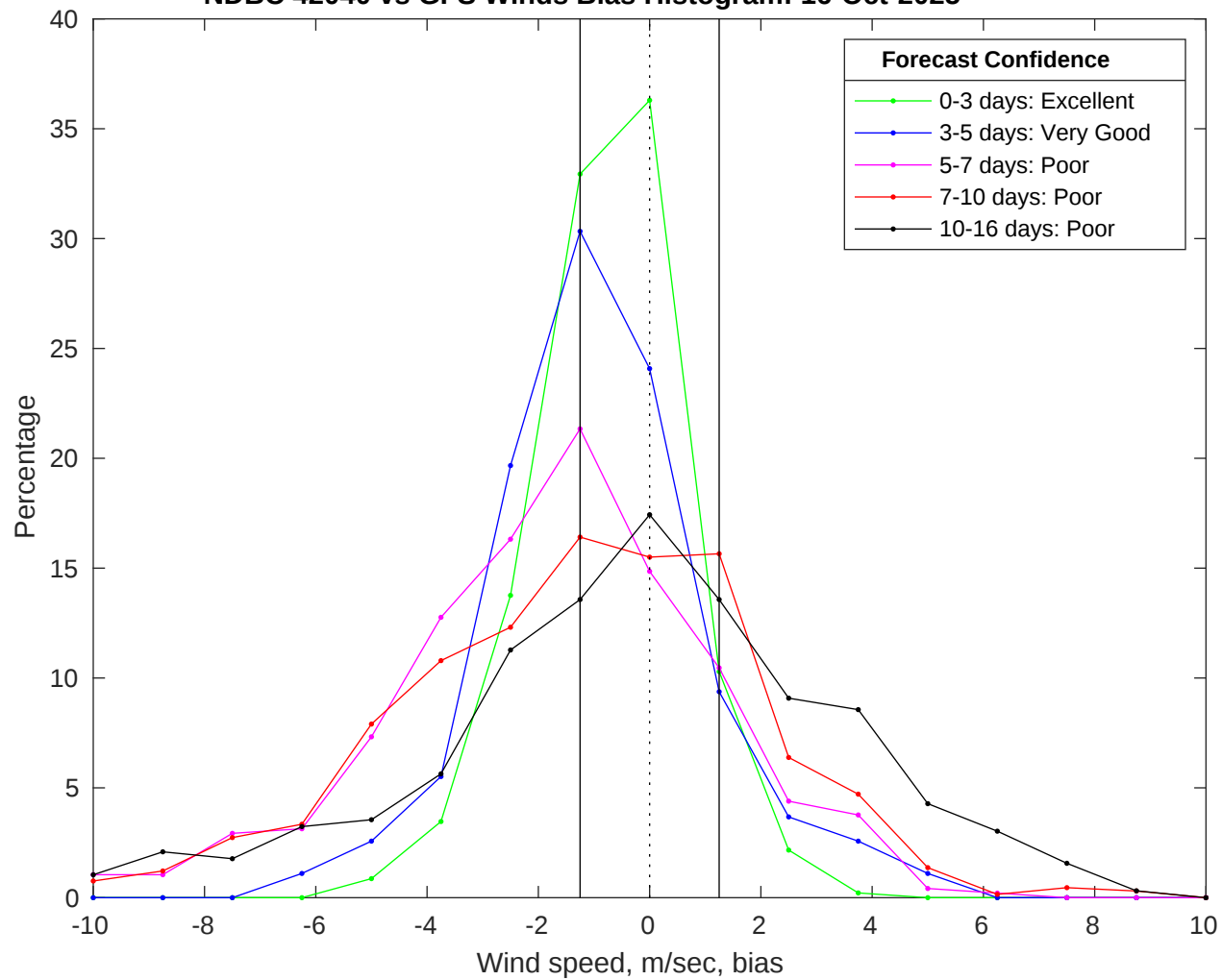
NDBC 42040 vs GFS Winds Bias Histogram: 16-Oct-2025
