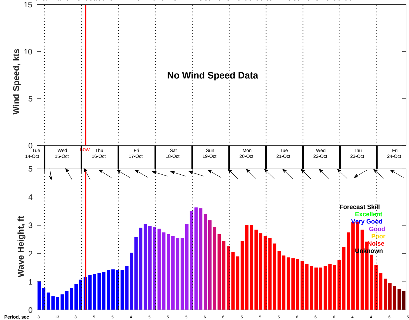
Wind & Wave Forecast for NDBC 42040 from 14-Oct-2025 19:00:00 to 24-Oct-2025 19:00:00
