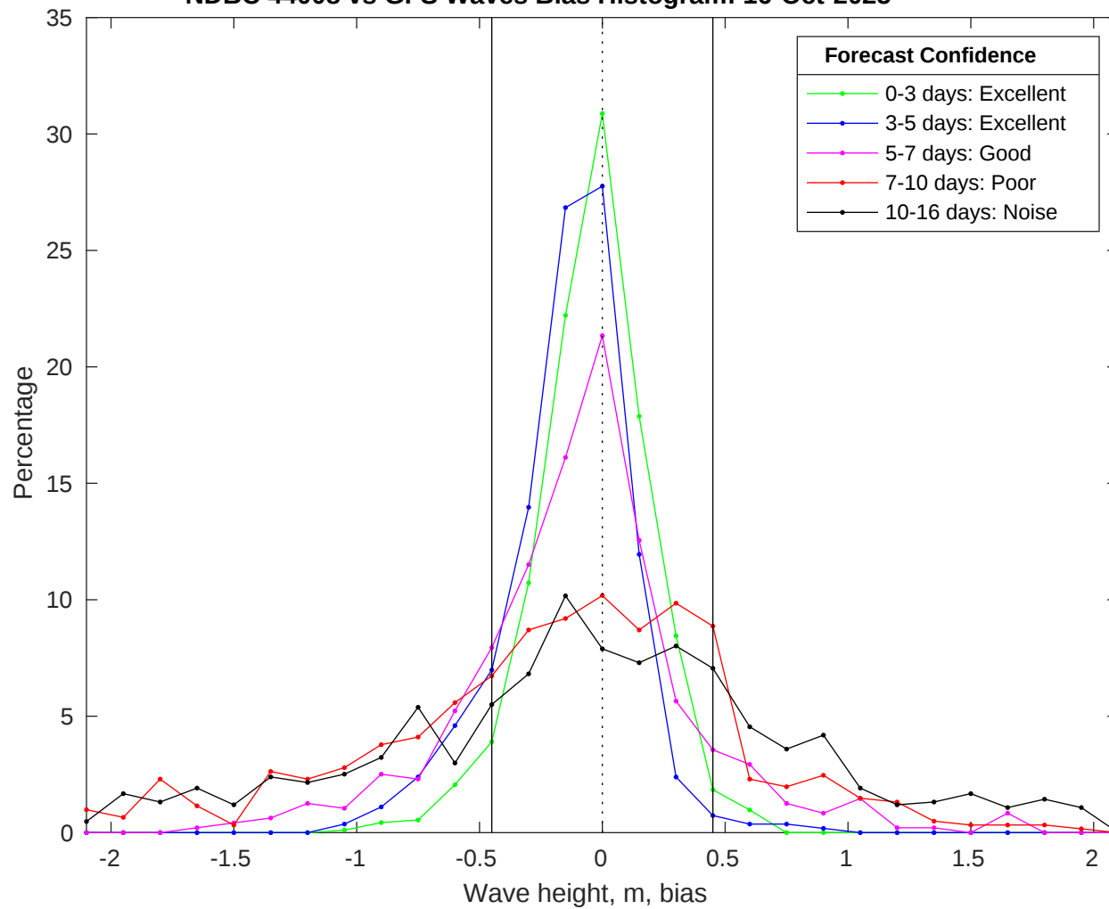
NDBC 44008 vs GFS Waves Bias Histogram: 16-Oct-2025
