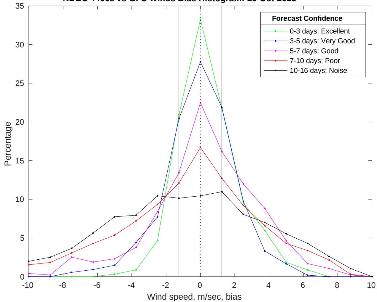
NDBC 44008 vs GFS Winds Bias Histogram: 16-Oct-2025
