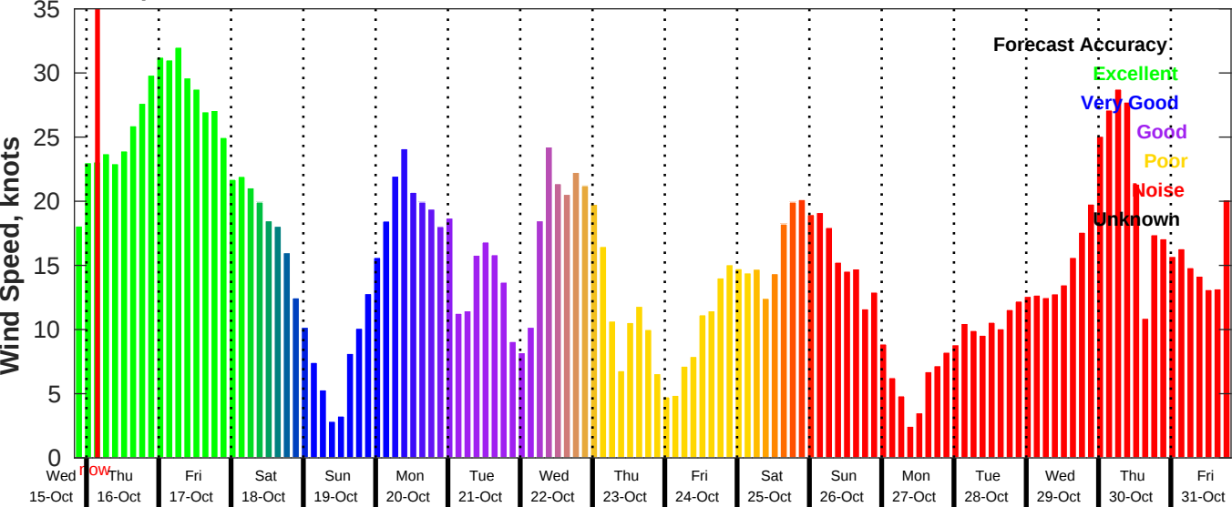
GFS Wind Speed Forecast for NDBC 44008 from 15-Oct-2025 20:00:00 to 31-Oct-2025 20:00:00
