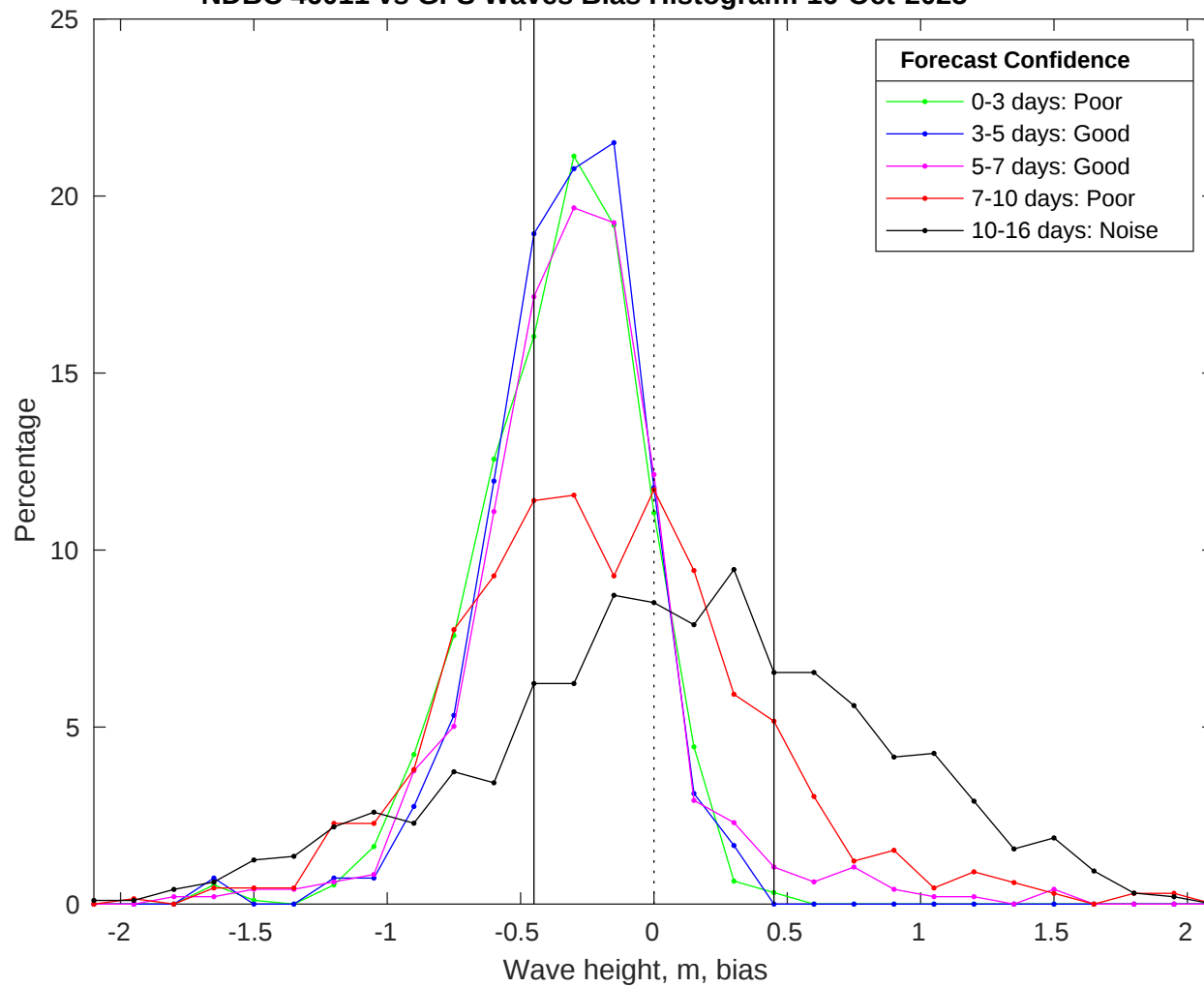
NDBC 46011 vs GFS Waves Bias Histogram: 16-Oct-2025
