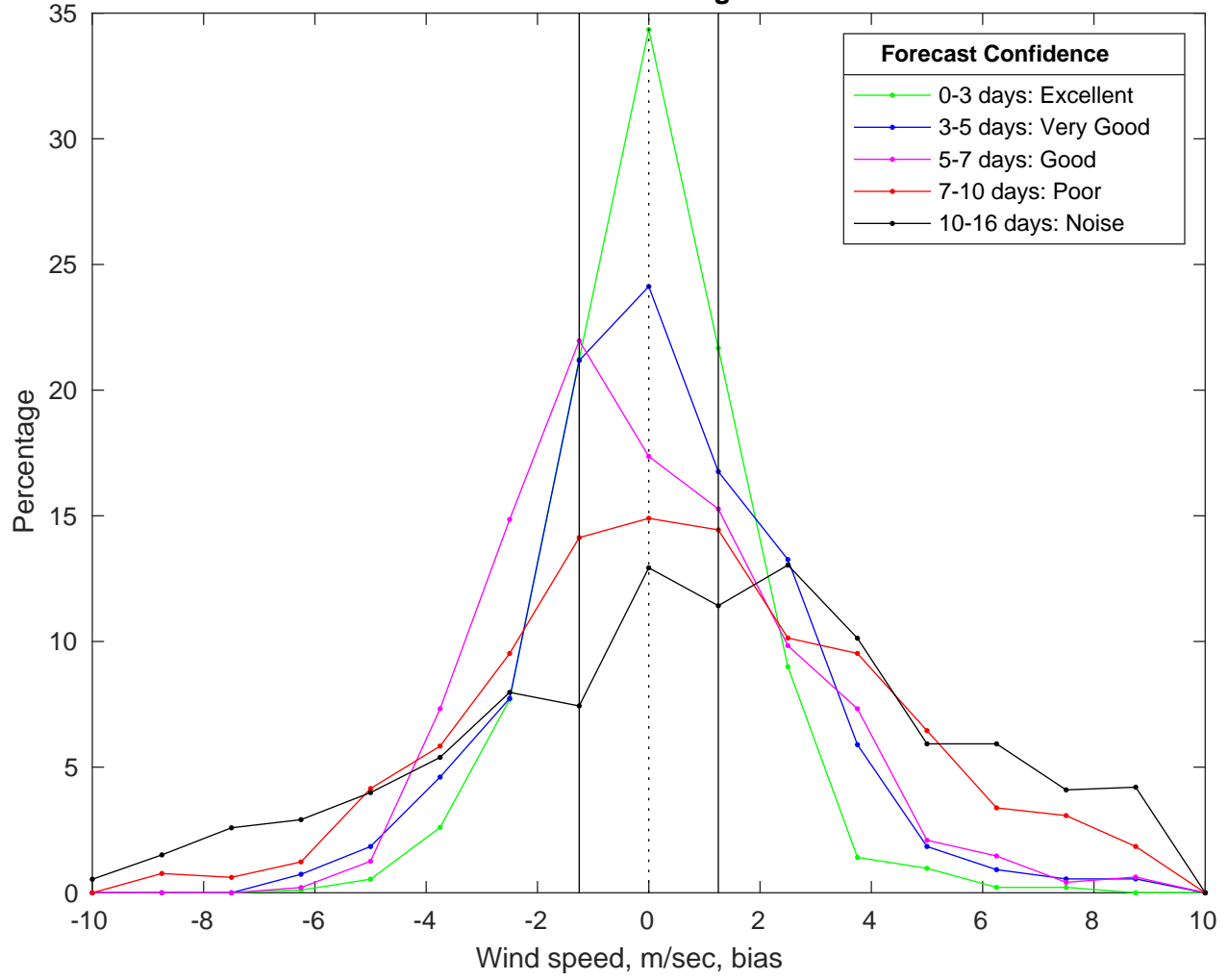
NDBC 46011 vs GFS Winds Bias Histogram: 16-Oct-2025
