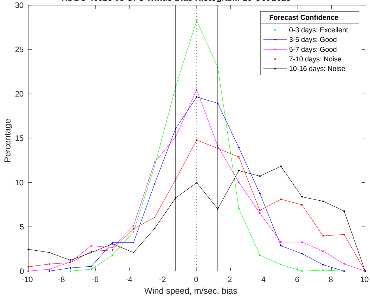
NDBC 46028 vs GFS Winds Bias Histogram: 16-Oct-2025
