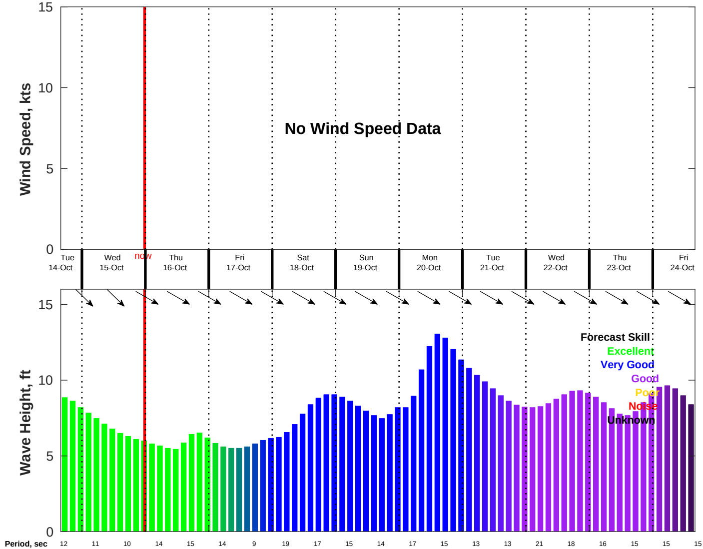
Wind & Wave Forecast for NDBC 46028 from 14-Oct-2025 16:00:00 to 24-Oct-2025 16:00:00
