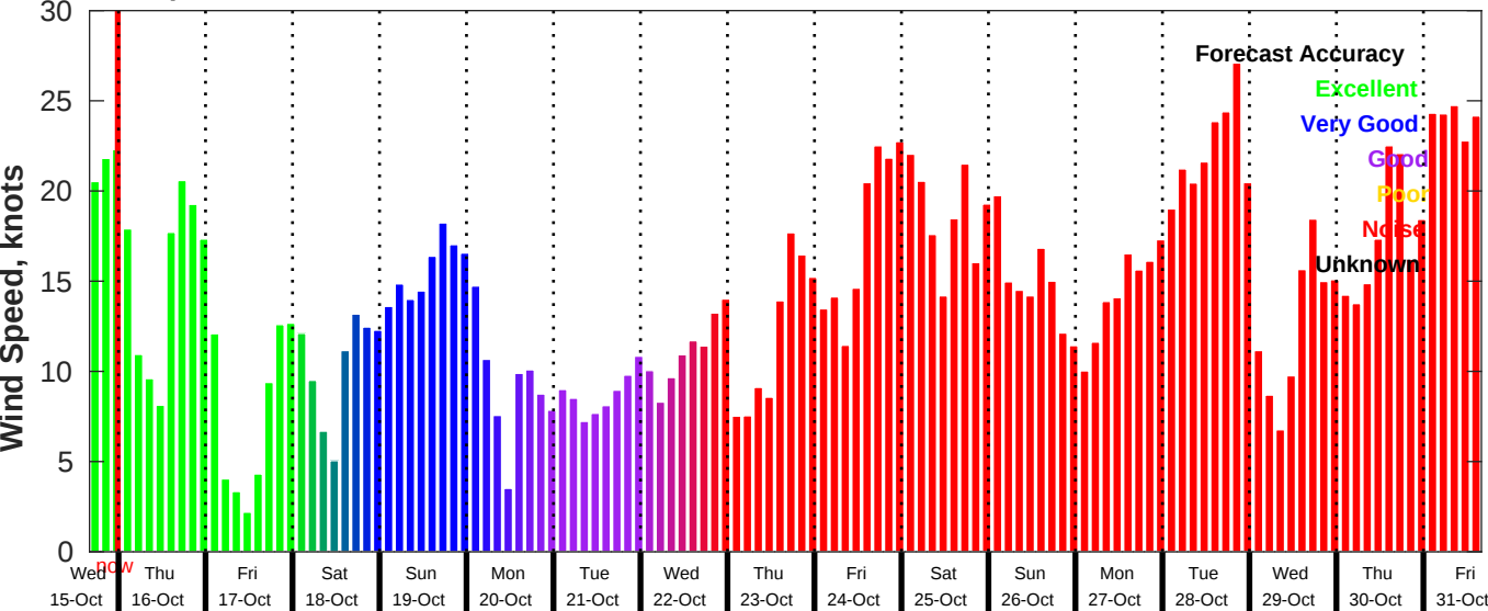
GFS Wind Speed Forecast for NDBC 46054 from 15-Oct-2025 16:00:00 to 31-Oct-2025 16:00:00
