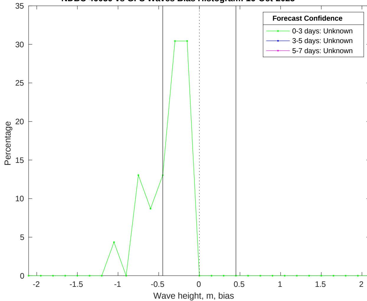
NDBC 46059 vs GFS Waves Bias Histogram: 16-Oct-2025
