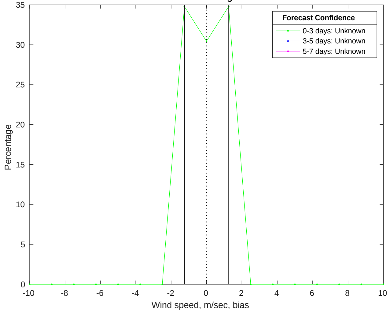
NDBC 46059 vs GFS Winds Bias Histogram: 16-Oct-2025
