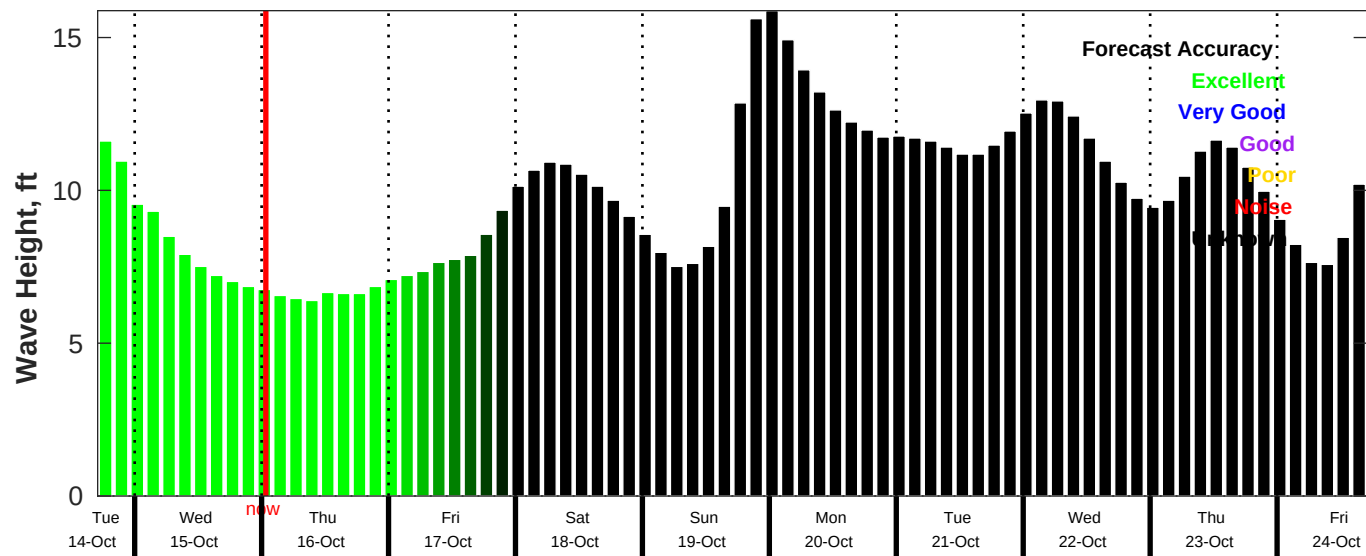
CMEMS Wave Forecast for NDBC 46059 from 14-Oct-2025 17:00:00 to 24-Oct-2025 17:00:00
