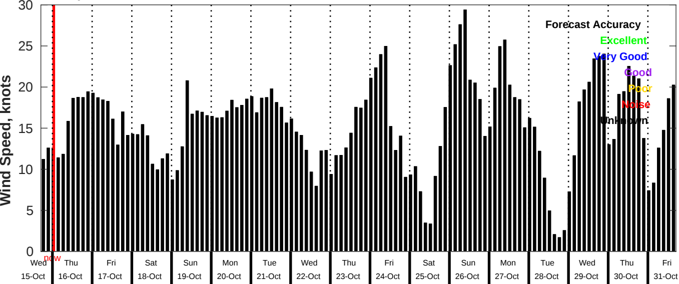
GFS Wind Speed Forecast for NDBC 46059 from 15-Oct-2025 17:00:00 to 31-Oct-2025 17:00:00
