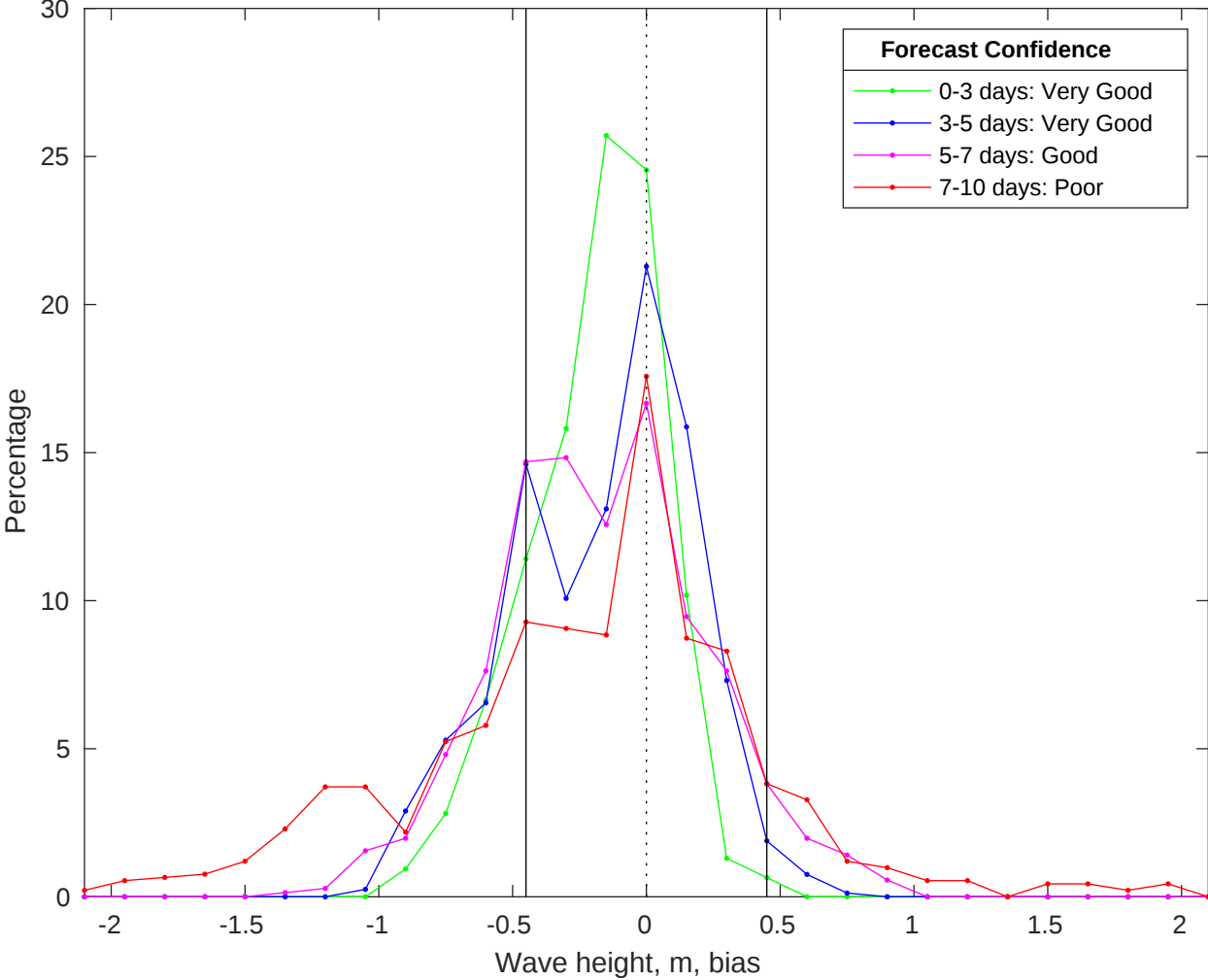
NDBC 46069 vs CMEMS Waves Bias Histogram: 16-Oct-2025
