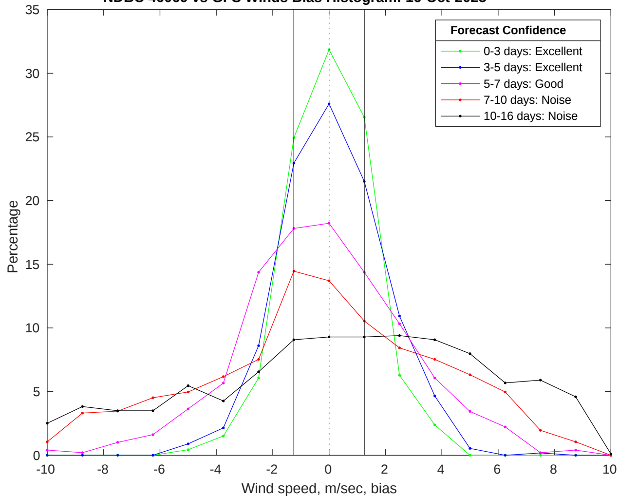
NDBC 46069 vs GFS Winds Bias Histogram: 16-Oct-2025
