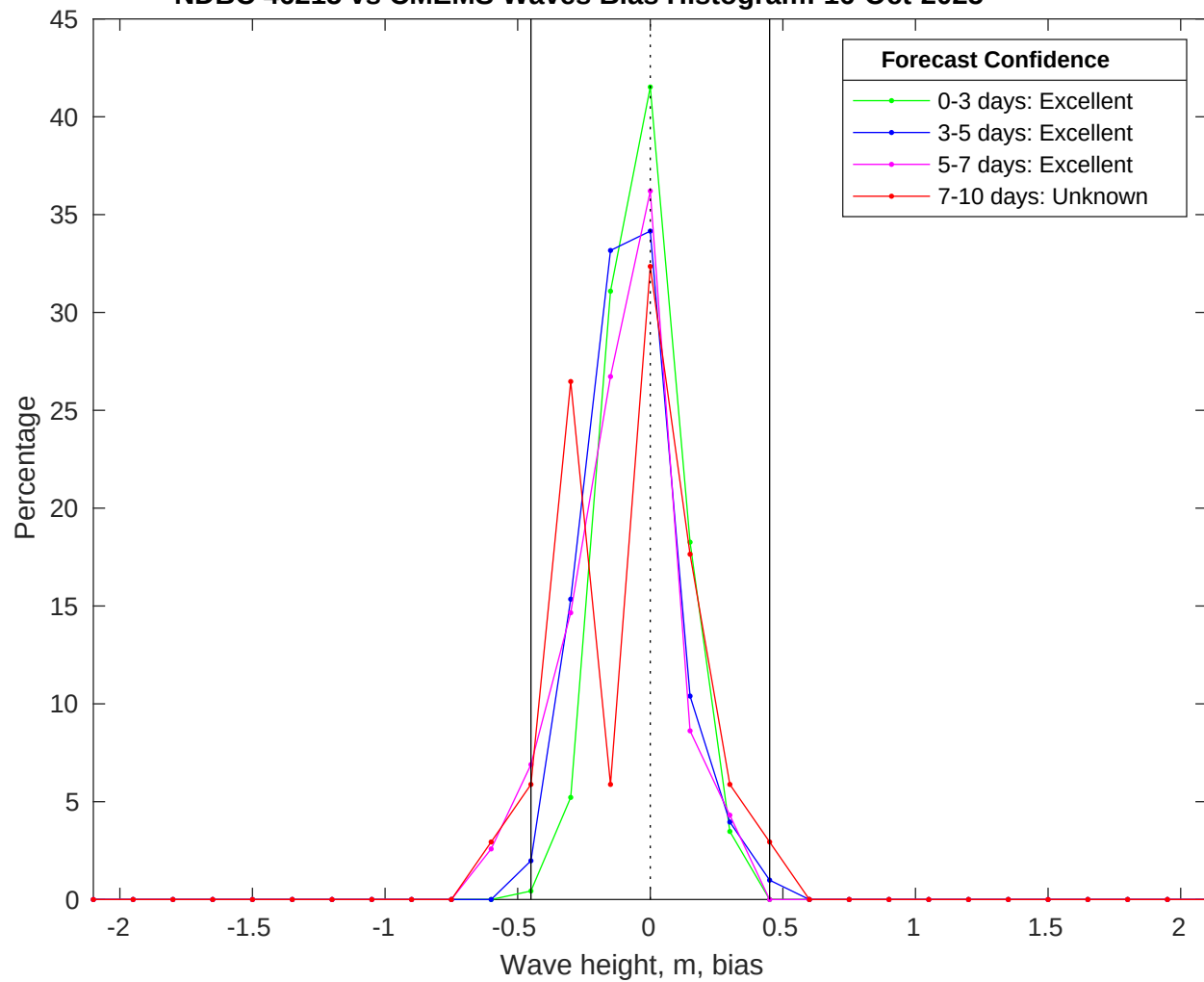
NDBC 46215 vs CMEMS Waves Bias Histogram: 16-Oct-2025
