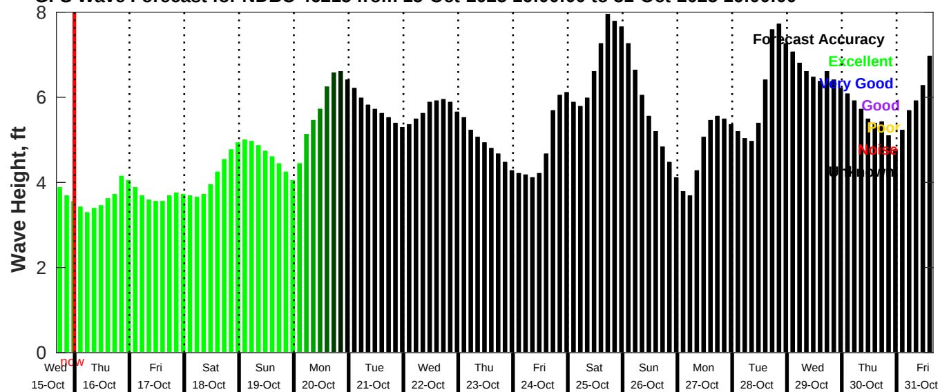
GFS Wave Forecast for NDBC 46215 from 15-Oct-2025 16:00:00 to 31-Oct-2025 16:00:00
