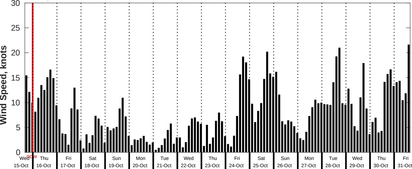
GFS Wind Speed Forecast for NDBC 46215 from 15-Oct-2025 16:00:00 to 31-Oct-2025 16:00:00
