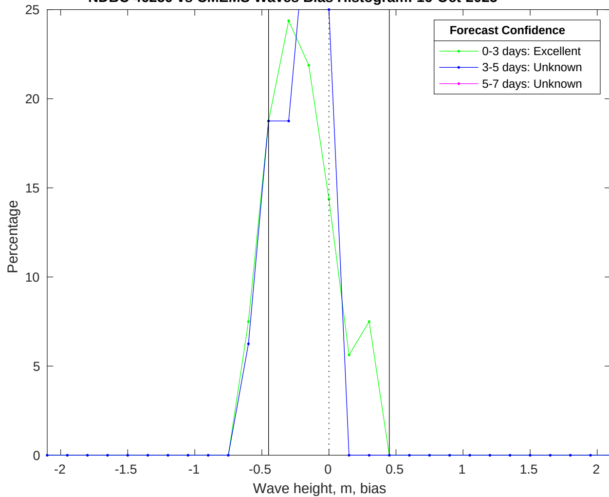
NDBC 46259 vs CMEMS Waves Bias Histogram: 16-Oct-2025
